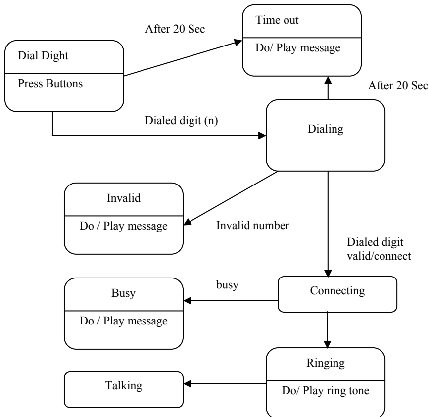
Figure 6: State Diagram for a Mobile
