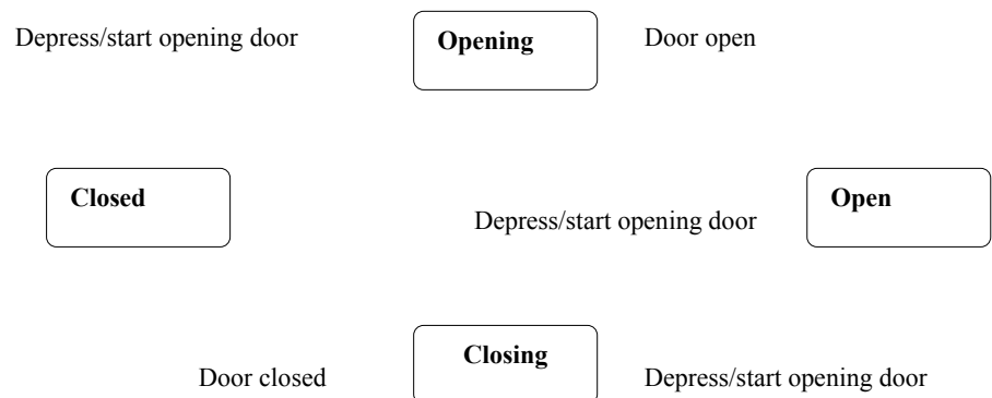
Figure 14: State diagram for a garage door opener
