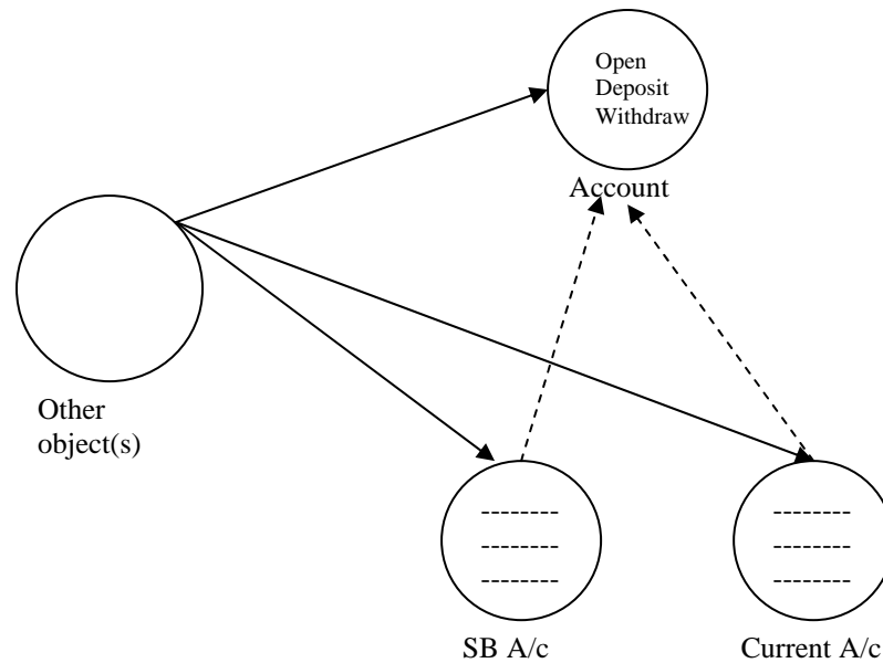
Figure 4: OO Decomposition (OOD)
