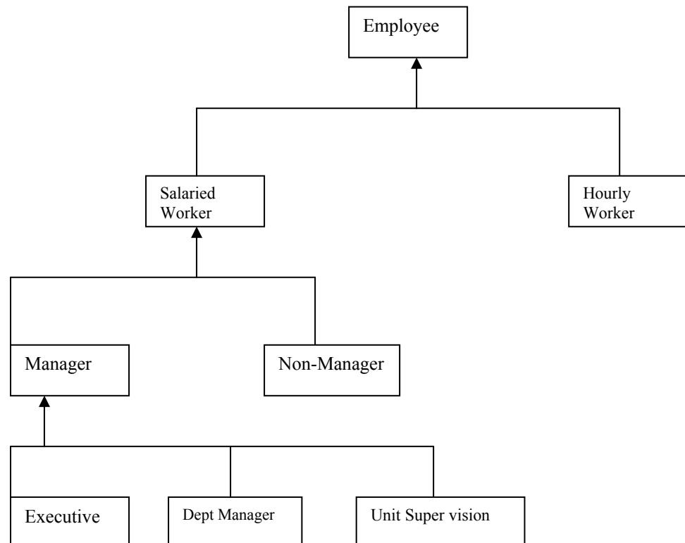
Figure 6: Generalization hierarchy of employee class
