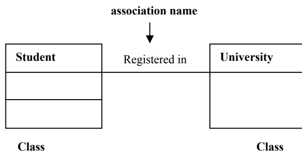
Figure 4a: Association
