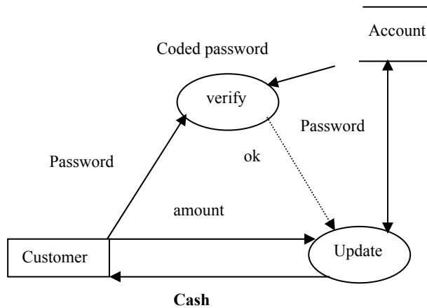
Figure 7: Control flow
