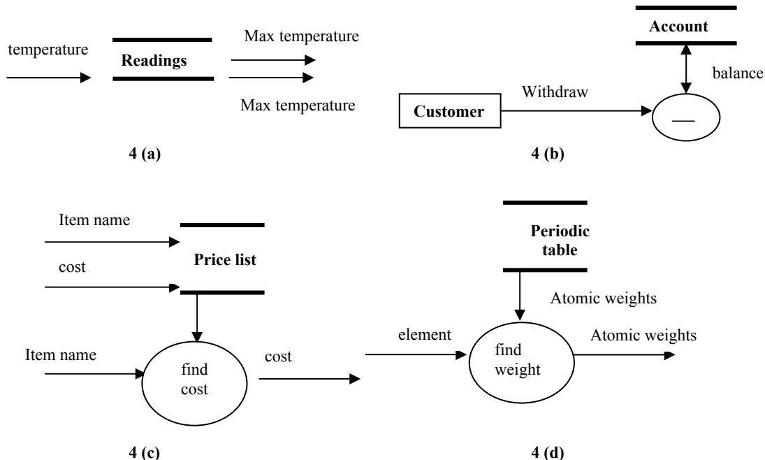
Figure 4: Data stores
