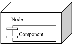
Figure 17: Deployment
