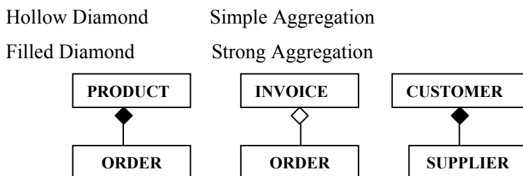
Figure 6: Aggregation
