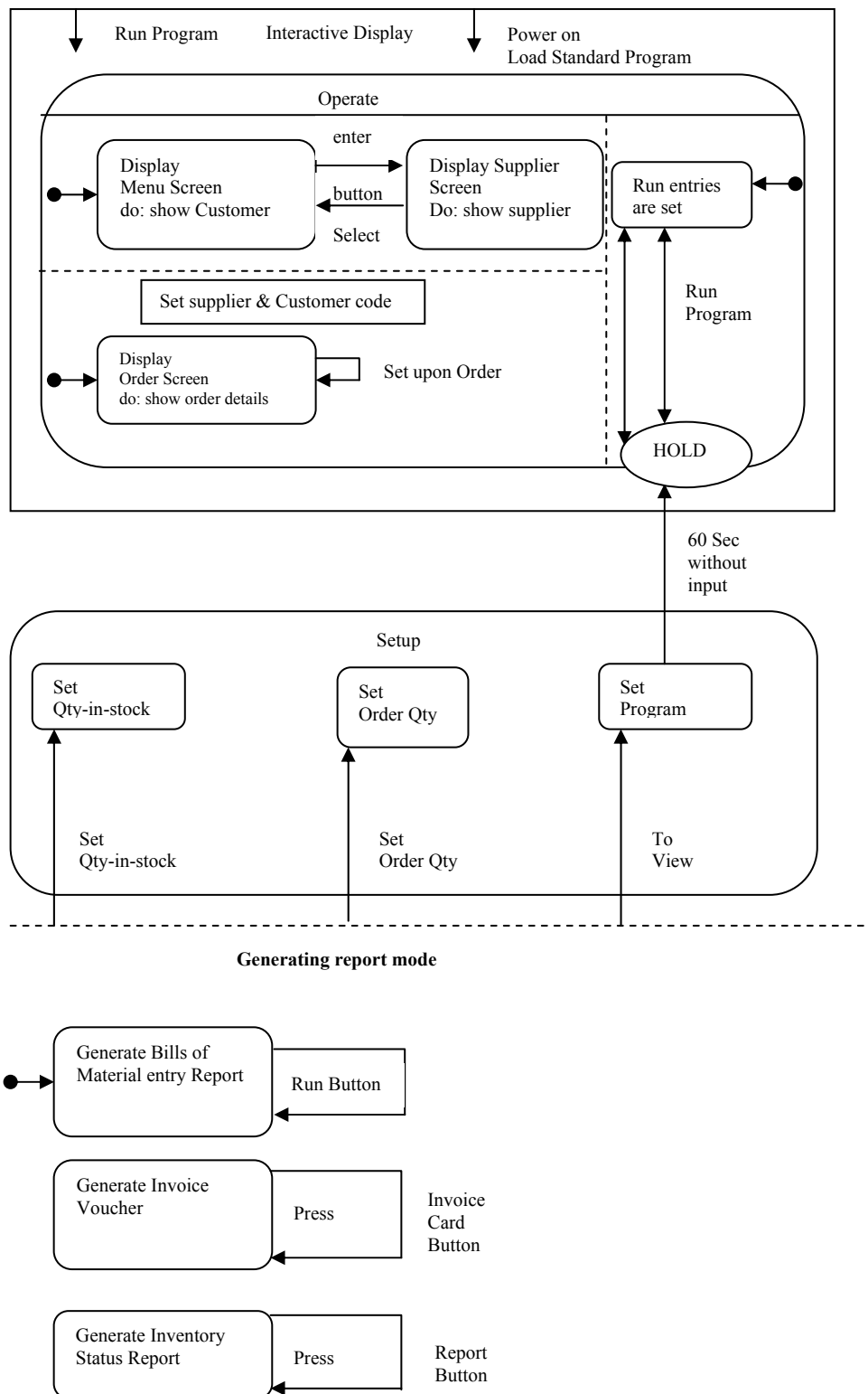
Figure 16: User interface
