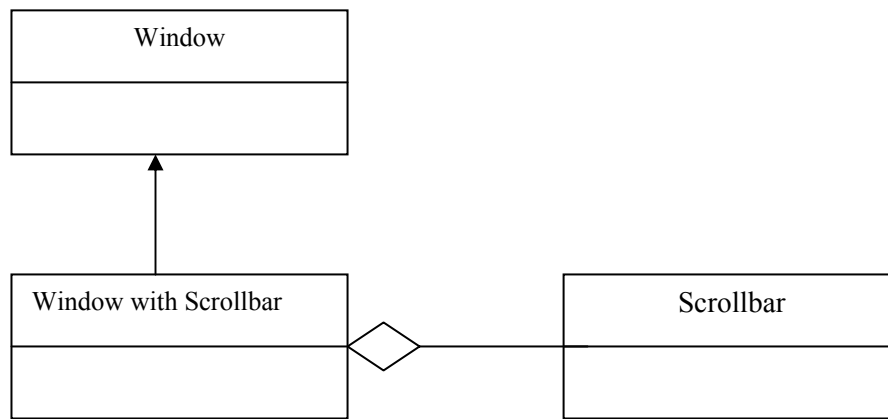
Figure 10: Class Diagram
