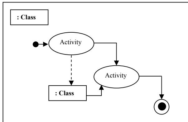
Figure 9: Activity flow
