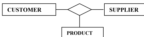
Figure 7: Ternary association
