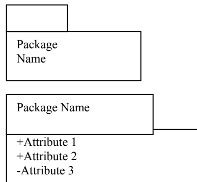
Figure 11: Package Diagram
