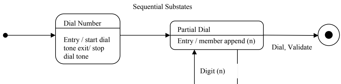
Figure 4: States Sequence
