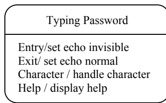
Figure 3: Entry-exit Action
