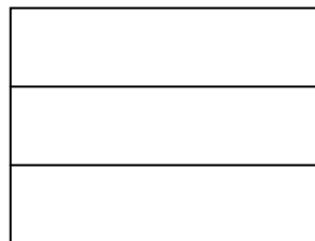
Figure 1: Class notation
