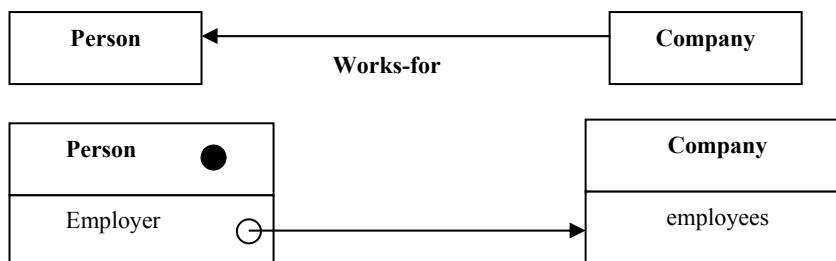
Figure 3: Implementation of one-way association using pointers
