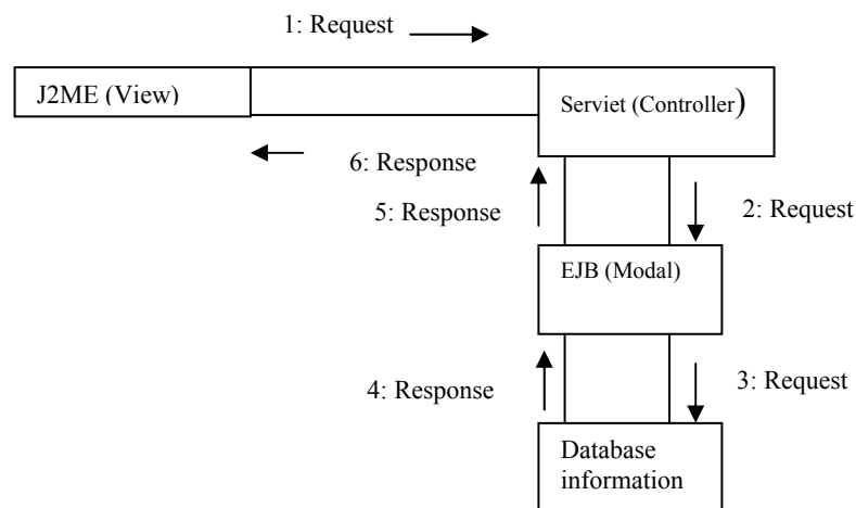
Figure 30: Collaboration diagram for execution using J2ME, Servlet and EJB
