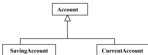
Figure 8: Generalization of account class
