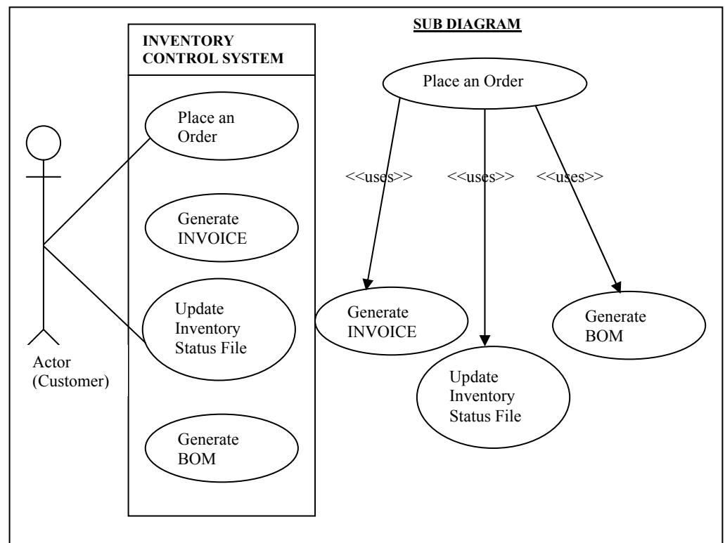
Figure 15: Initial design of the Inventory Control system
