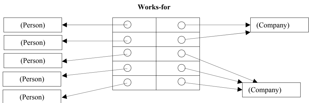
Figure 5: Implementation of association as an object
