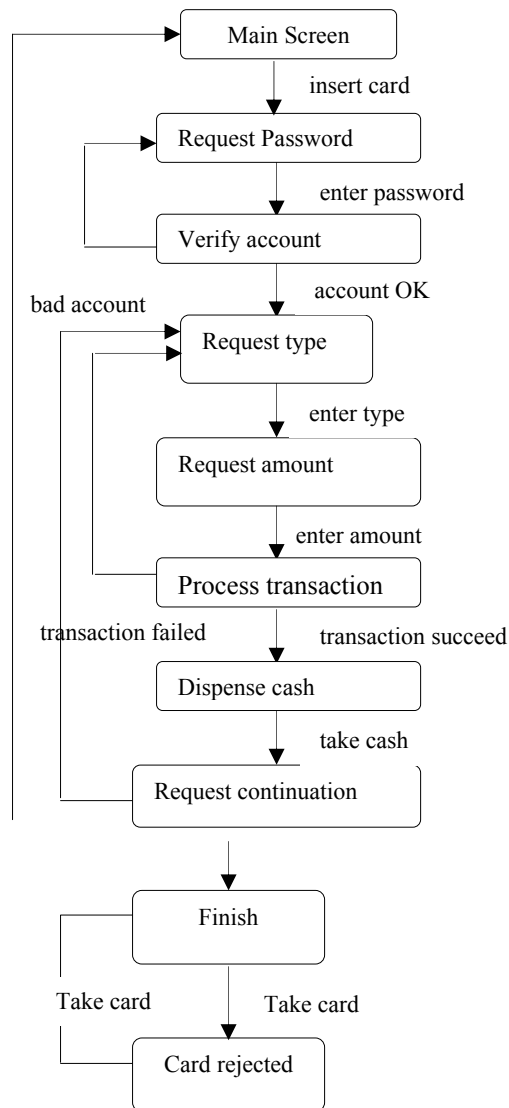
Figure 1: Control of states and events in ATM
