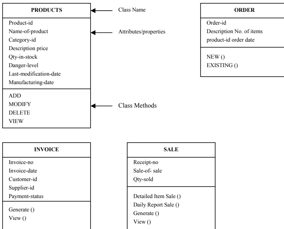
Figure 2: Class diagram
