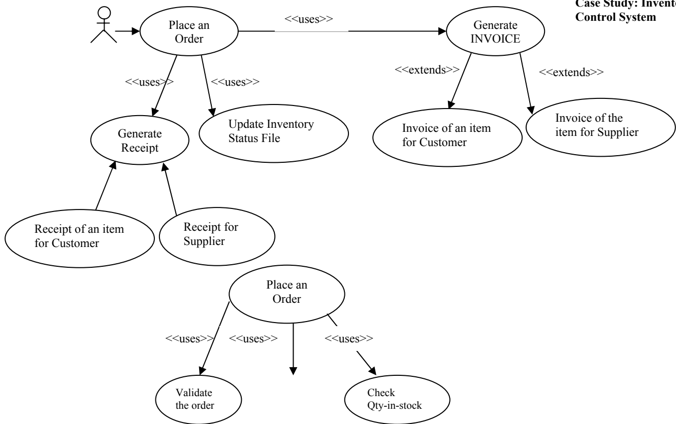
Figure 12: Adding details
