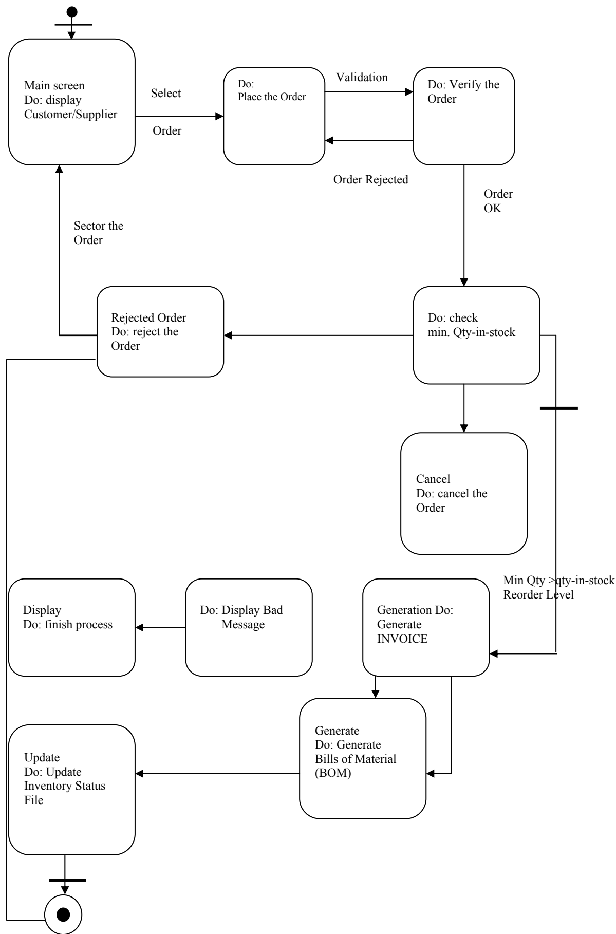
Figure 11: State diagram
