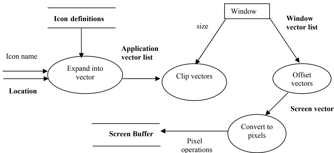
Figure 1: Data flow diagram for windowed graphics display
