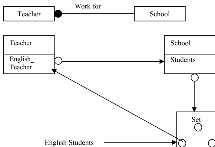
Figure 3: Implementation of two-way association, using pointer
