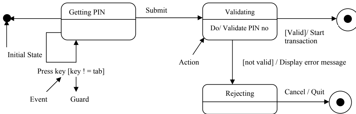
Figure 2: State chart diagram of login
