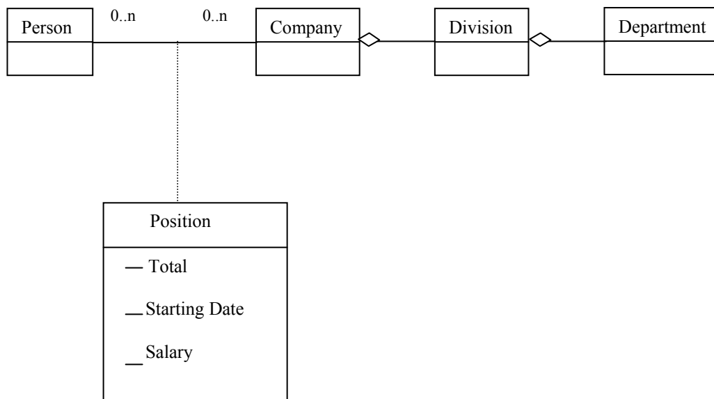
Figure 2: Example of a composition
