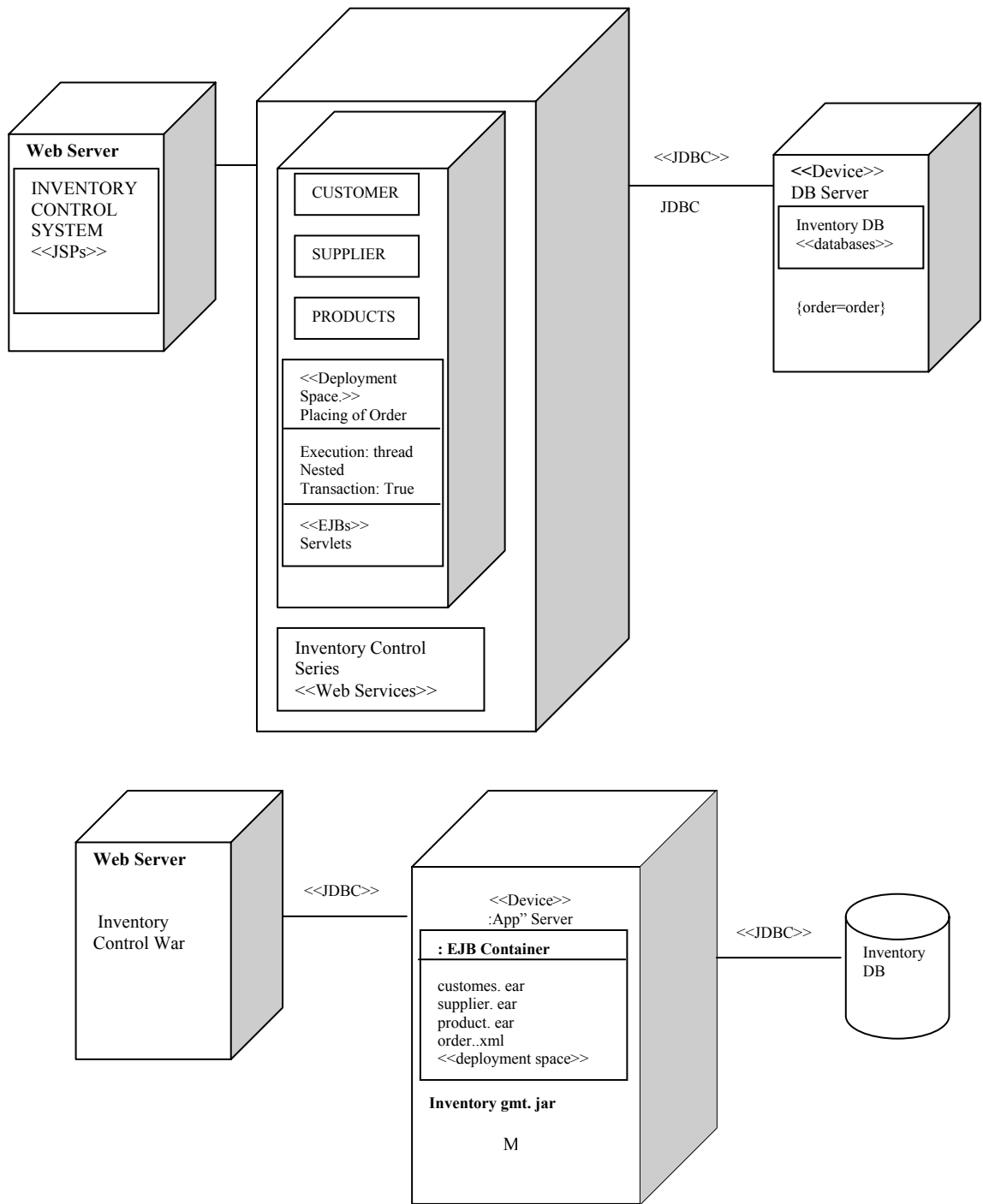
Figure 18: Deployment diagram
