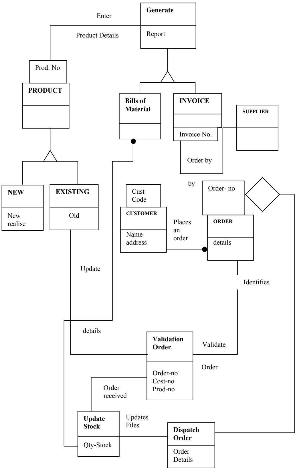
Figure 3: Object Diagram
