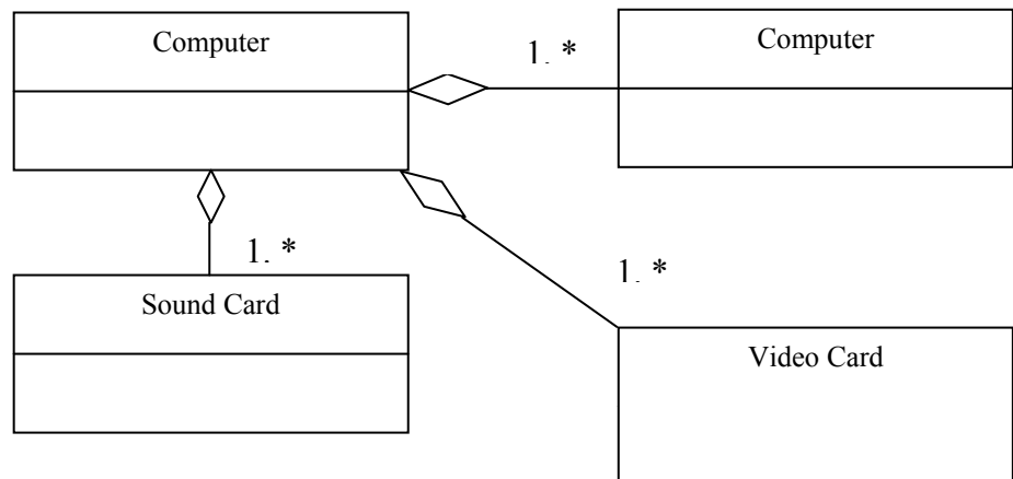
Figure 9: Class Diagram
