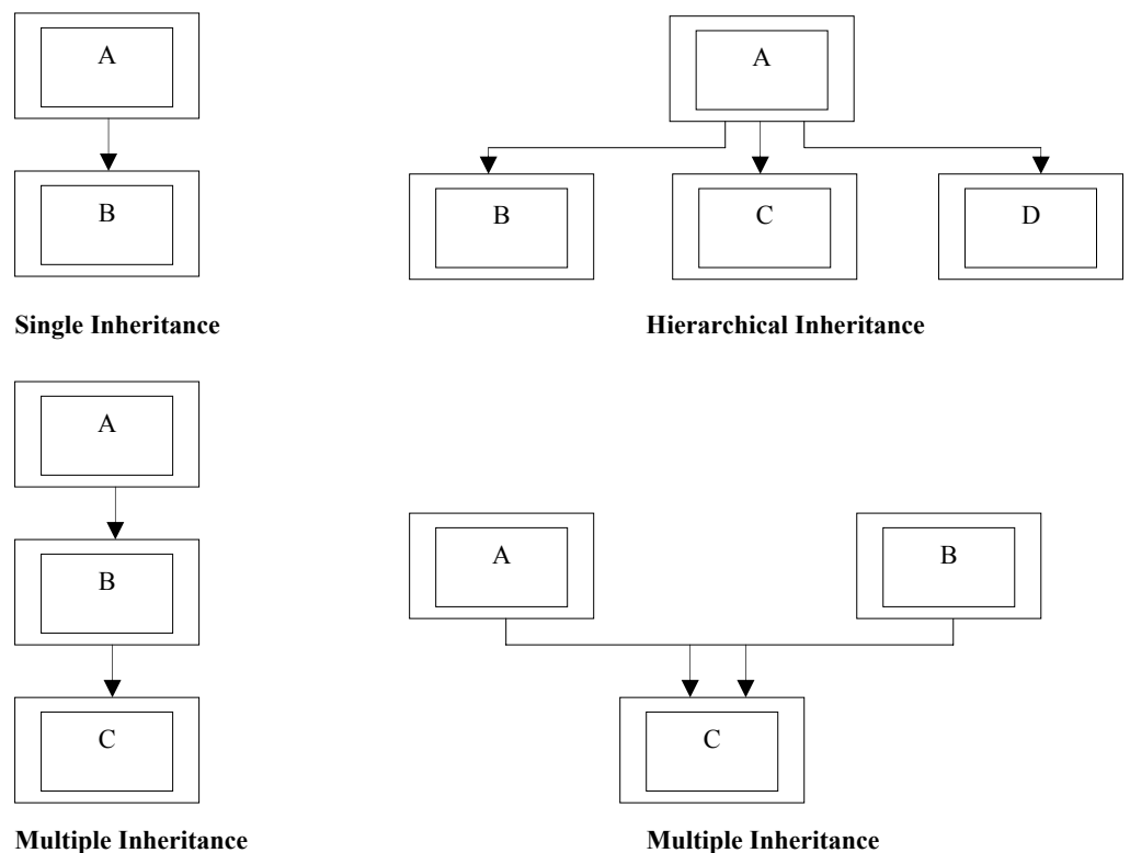
Figure 16: Forms of inheritance
