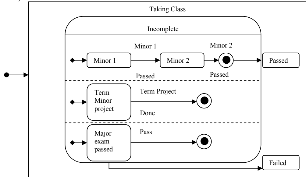
Figure 7: Concurrent Substate diagram
