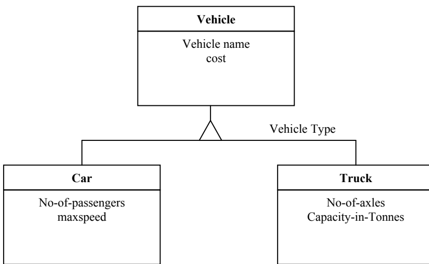
Figure 4: Object Model for Generalization
