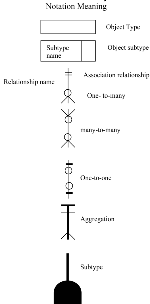
Figure 1: User Object Model Notations
