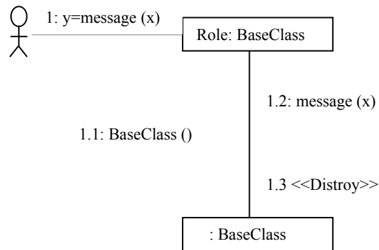
Figure 29: Collaboration diagram
