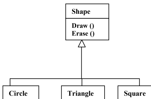
Figure 9: Single inheritance
