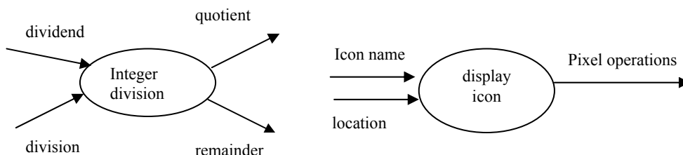
Figure 2: Processes
