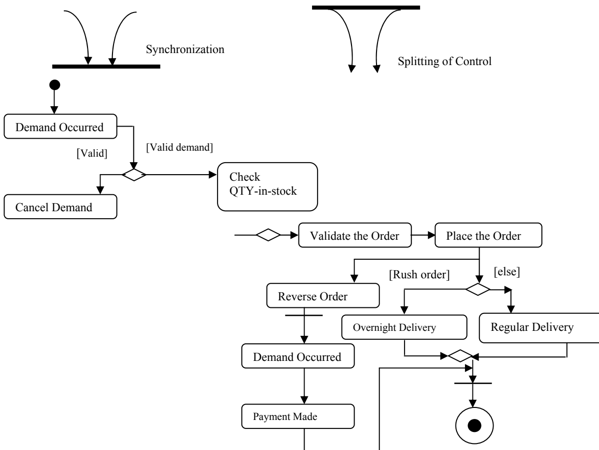
Figure 10: Activity diagram
