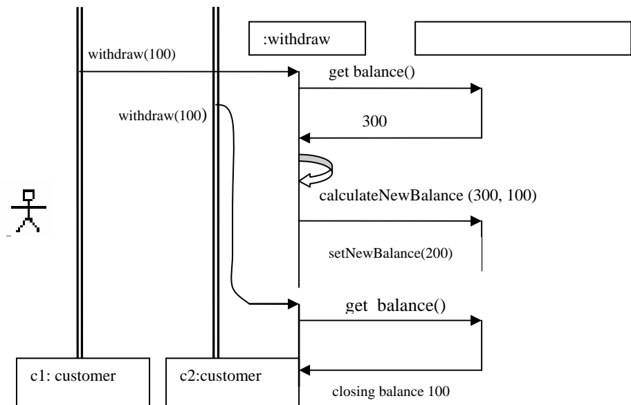
Figure 7: Concurrency with synchronization
