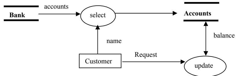
Figure 5: Selection with an object as result
