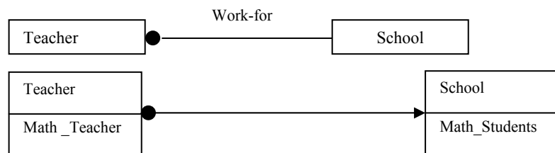
Figure 2: Implementation of a one-way association using pointers
