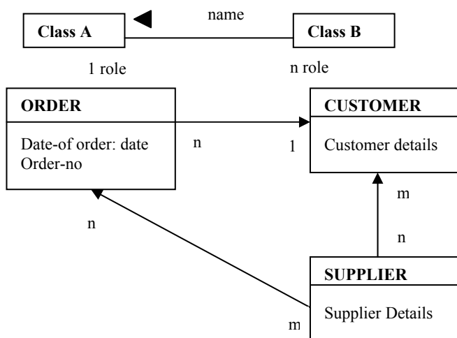
Figure 5: Association of Order and customer
