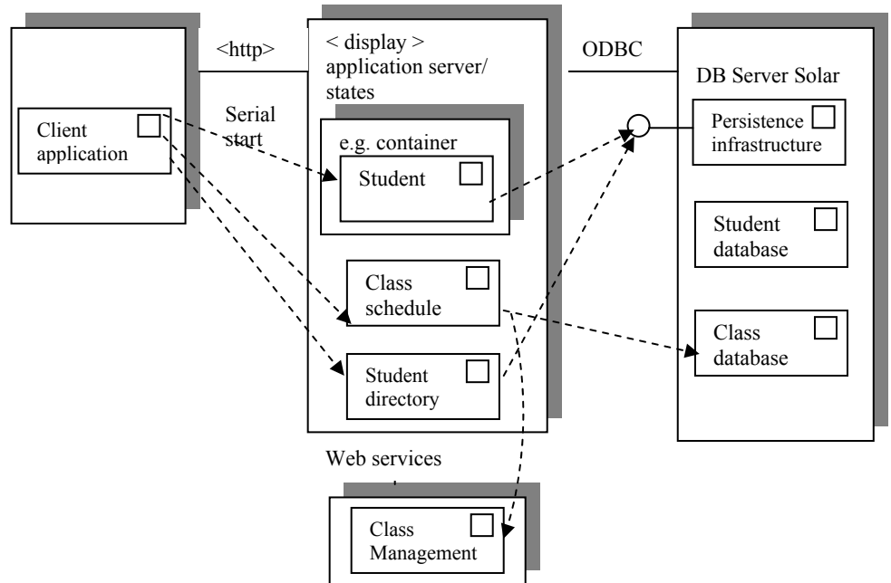
Figure 25: Deployment diagram for Student Administration
