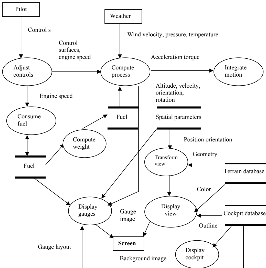
Figure 8: Functional model of flight simulator
