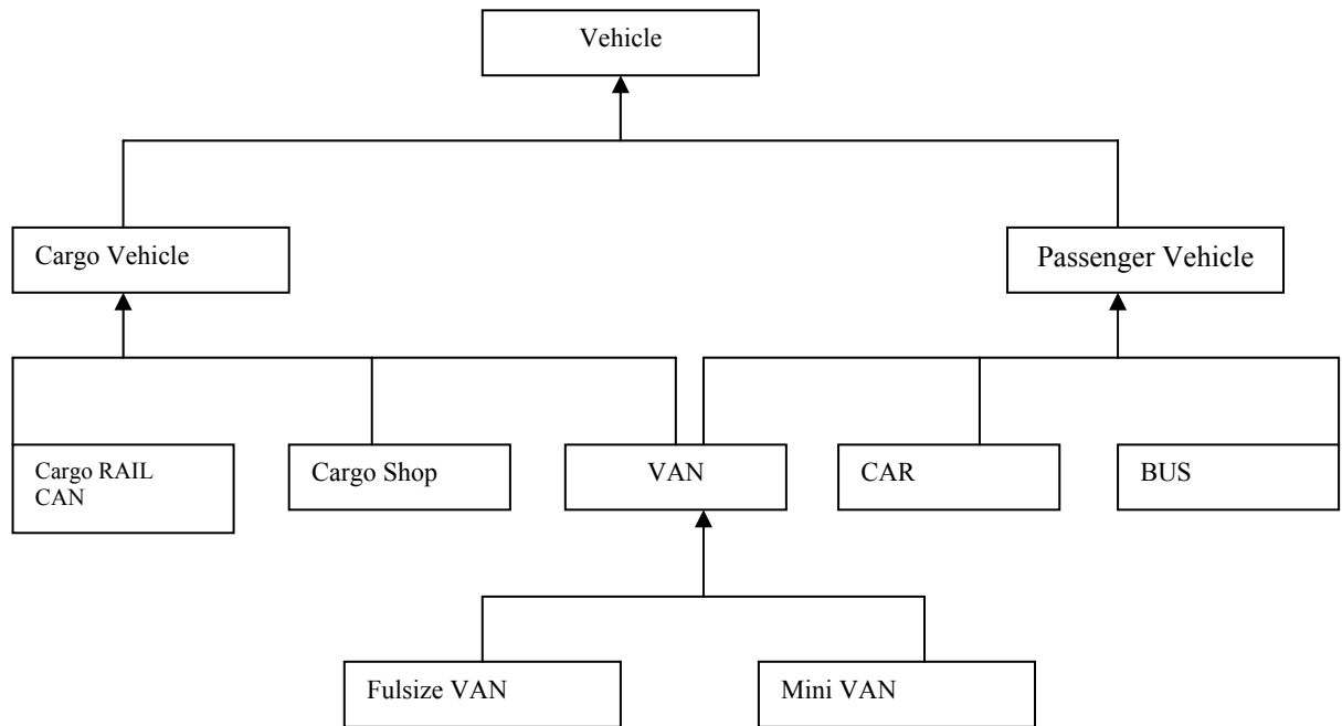
Figure 5: Example of Multiple Inheritance
