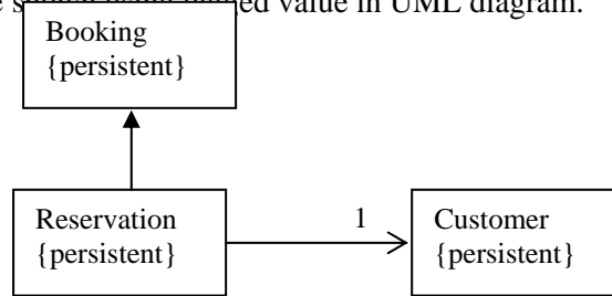
Figure 8: A UML diagram showing persistent class
