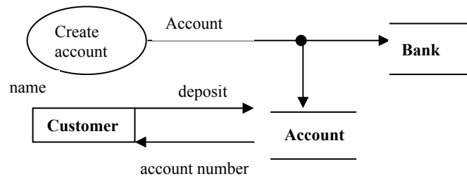
Figure 6: Creation of a new object
