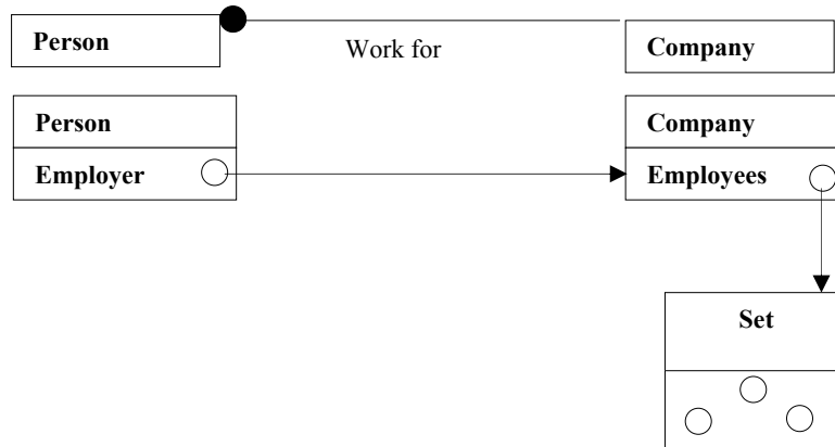
Figure 4: Implementation of two-way association using pointers
