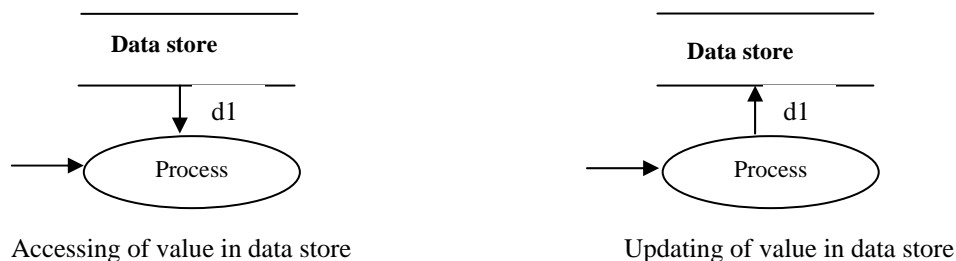
Figure 9: Functional Model notation of data store
