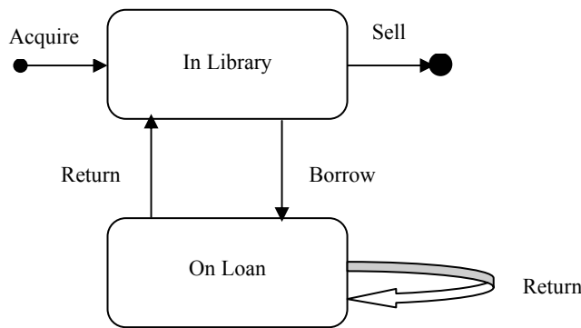
Figure 4: A simple State Diagram
