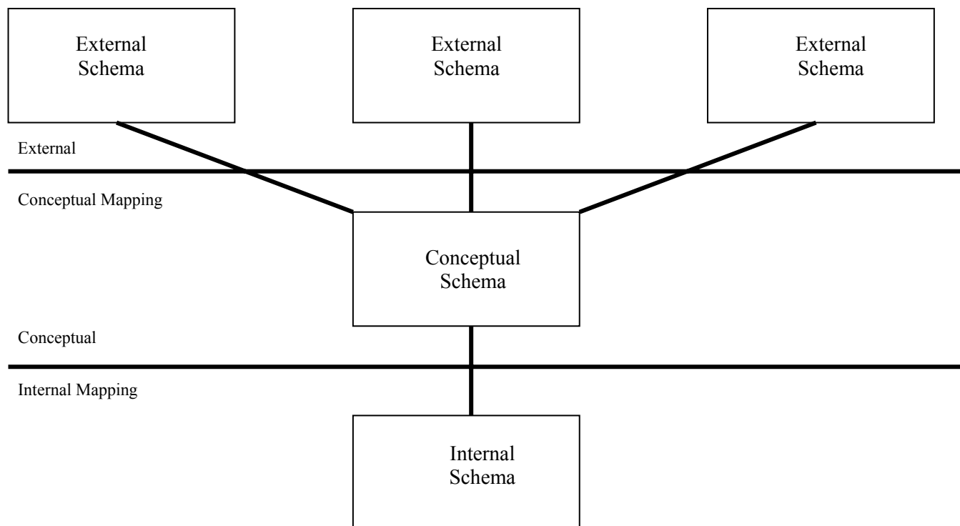
Figure 1: ANSI-SPARC Three level Architecture
