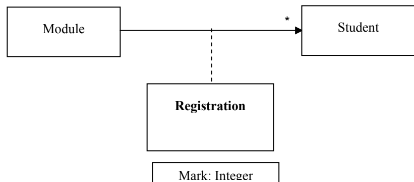
Figure 8: An association class
