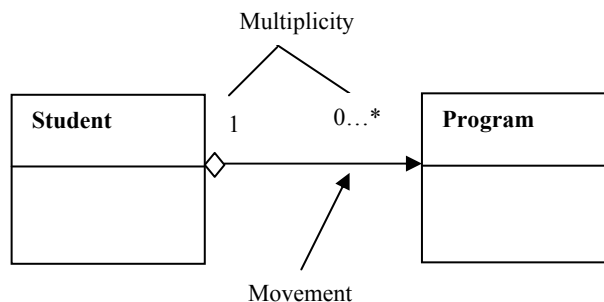
Figure 6: Association and movement
