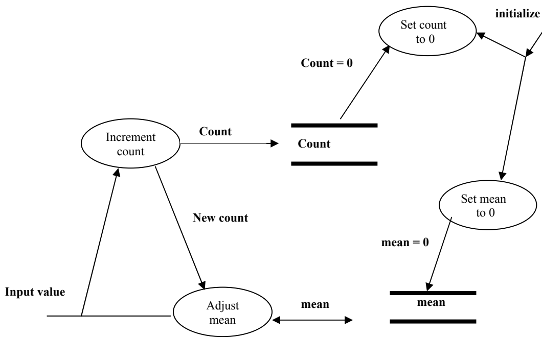
Figure 14 (a): DFD for computing mean
