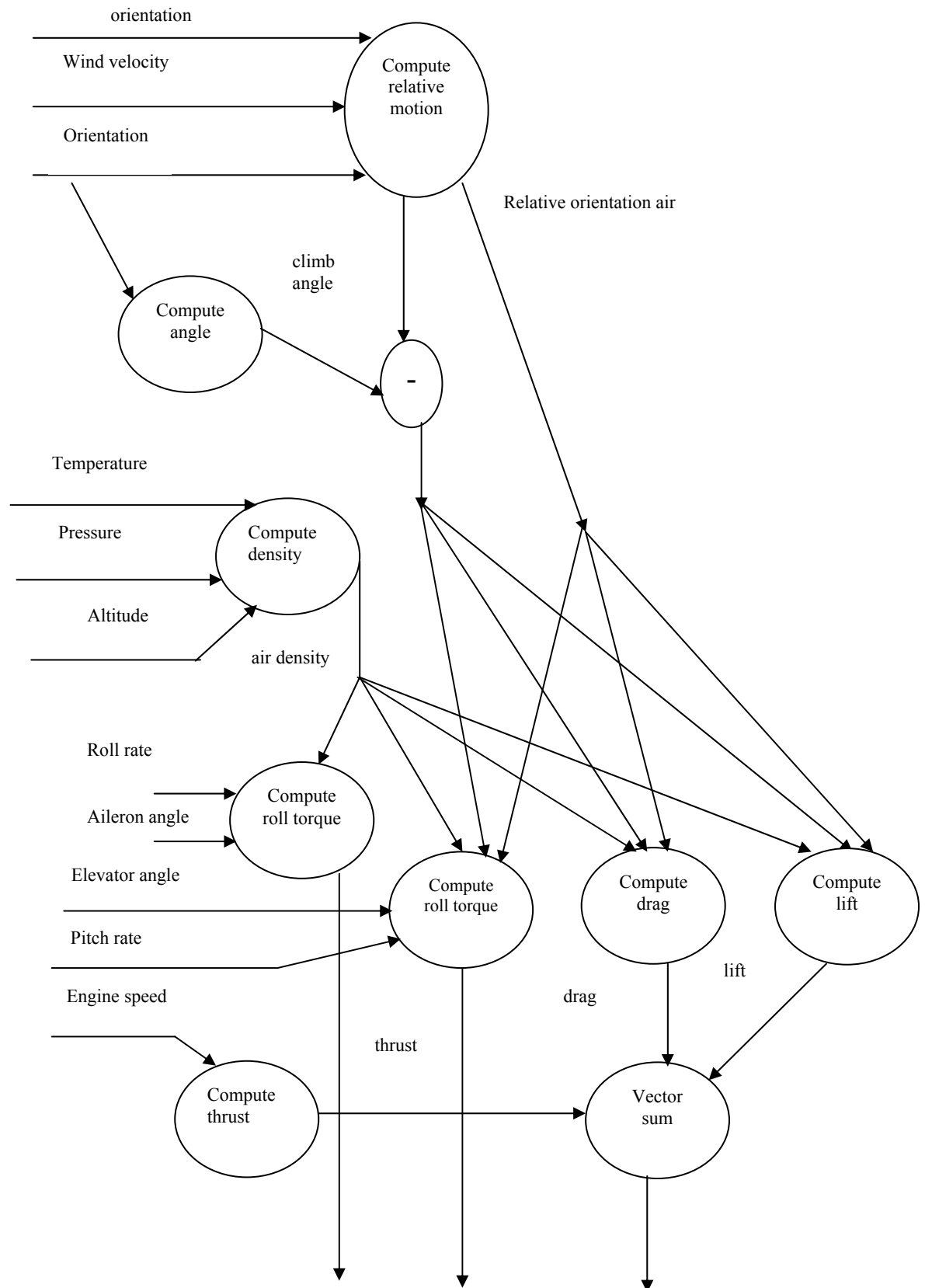
Figure 10: Expansion of compute forces processes
