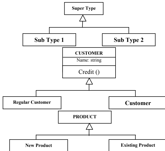
Figure 4: Generalisation of customer and product
