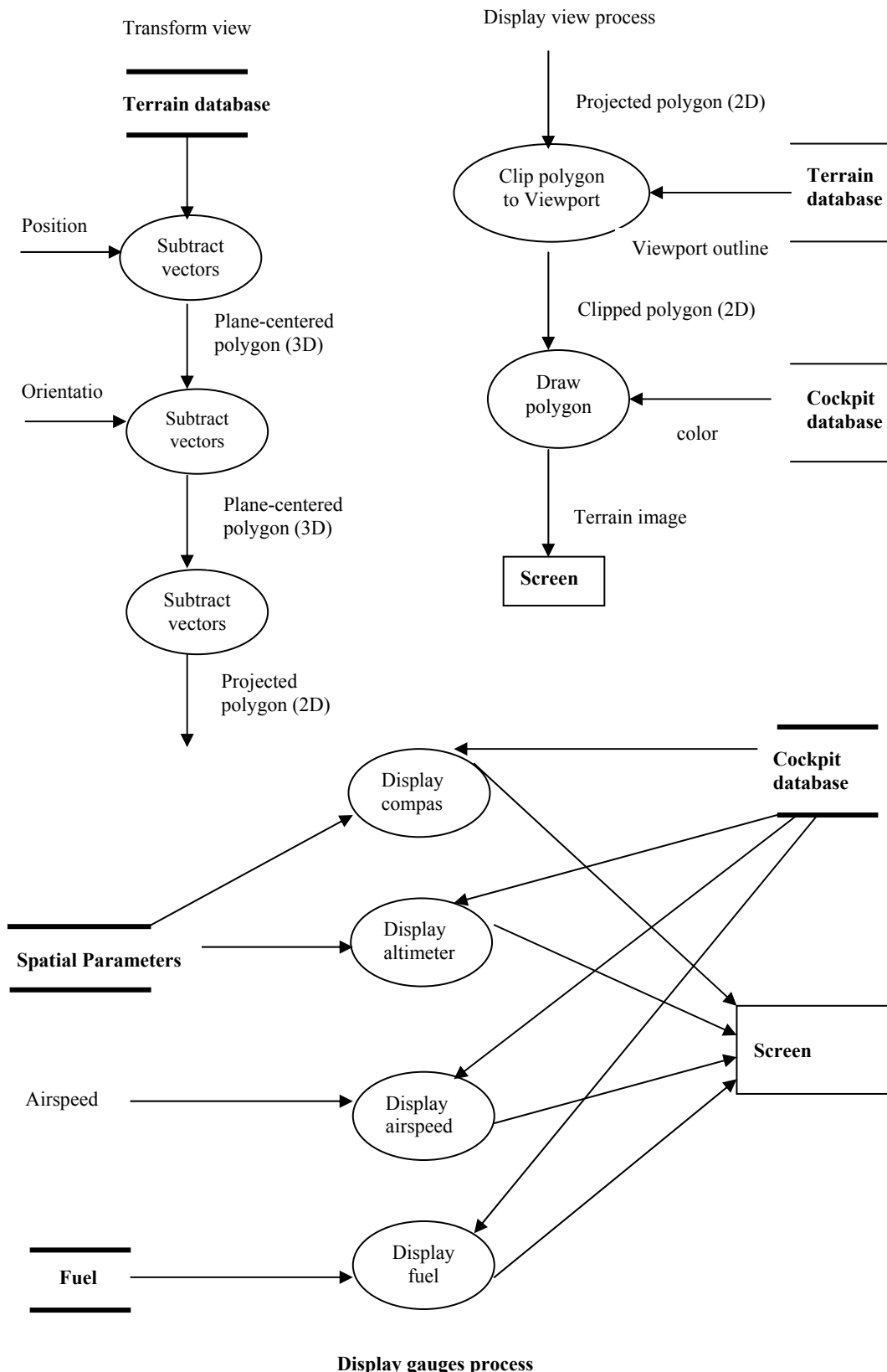
Figure 11: Expansion of display processes
